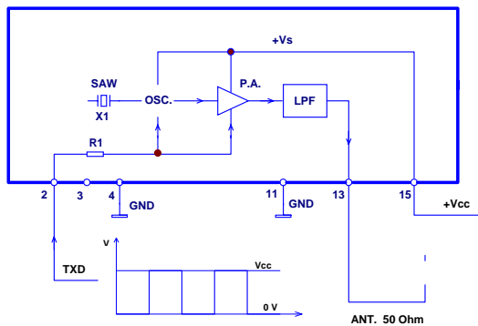
Fig.1 – BT27 BLOCK DIAGRAM.
