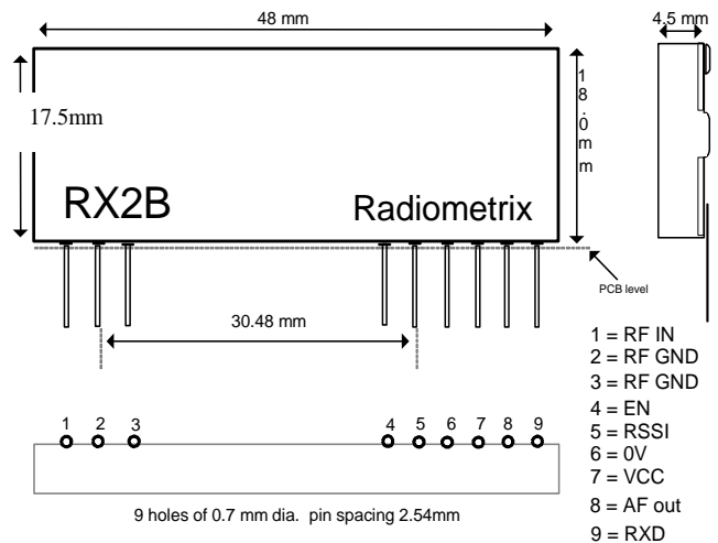
Figure 5: Physical dimensions
